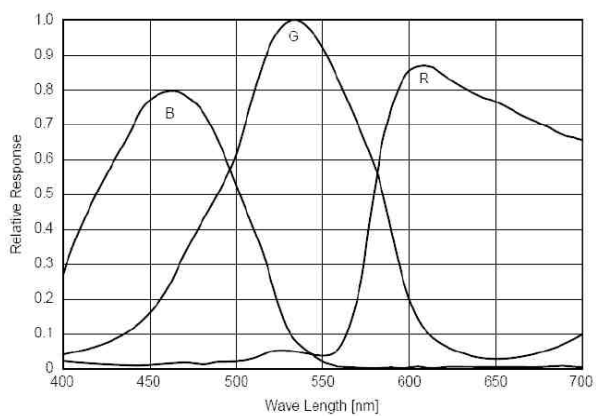
Spectral Response Guppy F-033C
