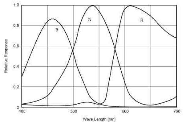
Spectral Response Guppy F-146C
