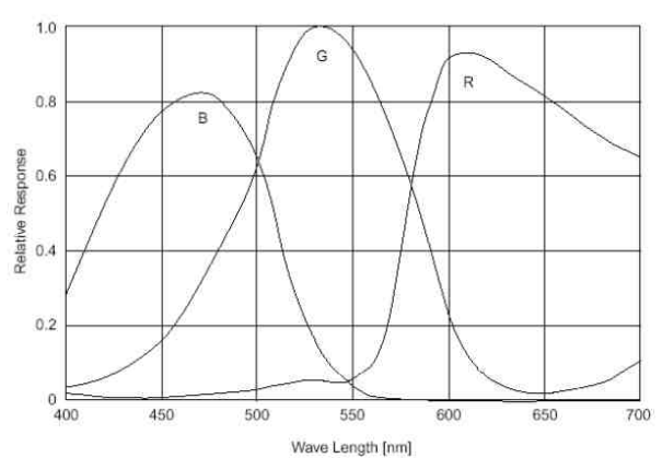
Spectral Response Guppy F-046C
