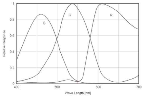
Spectral Response Guppy F-080C
