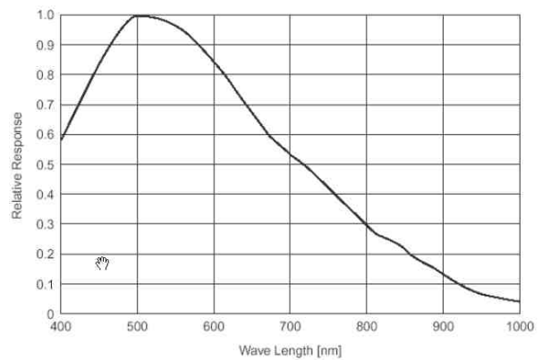
Spectral Response Guppy F-046B
