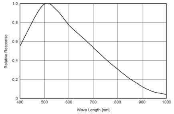
Spectral Response Guppy F-146B
