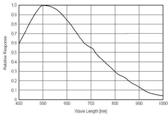
Spectral Response Guppy F-033B
