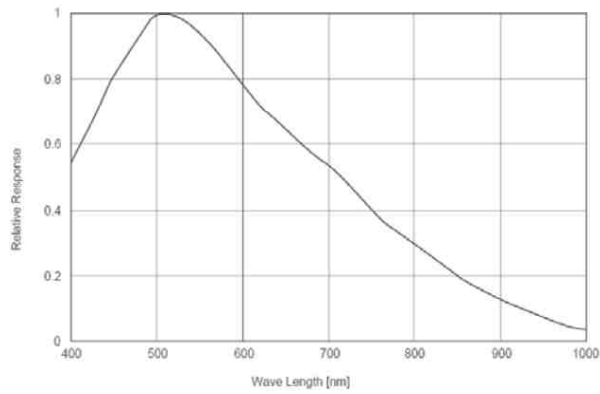
Spectral Response Guppy F-080B
