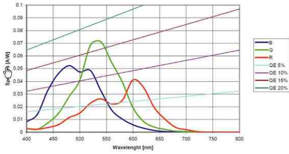
Spectral Response Marlin F131C
