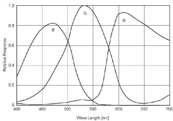
Spectral Response Marlin F033C
