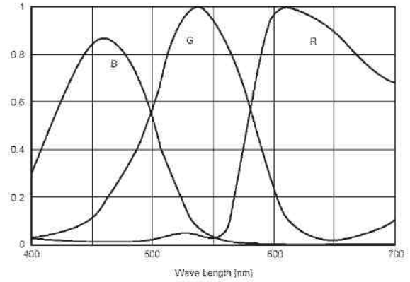
Spectral Response Marlin F146C
