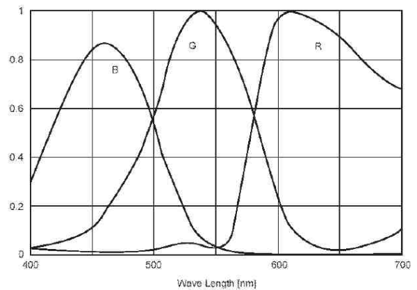
Spectral Response Marlin F080C
