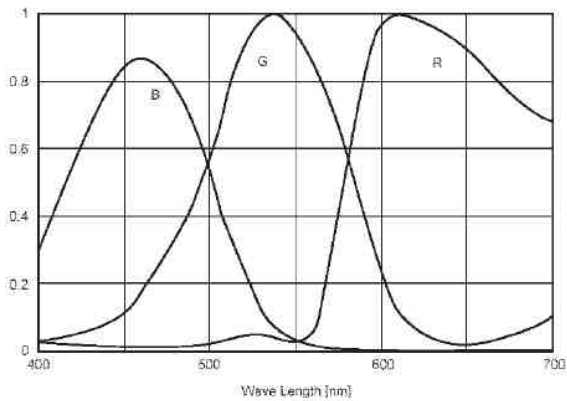
Spectral Response Marlin F201C
